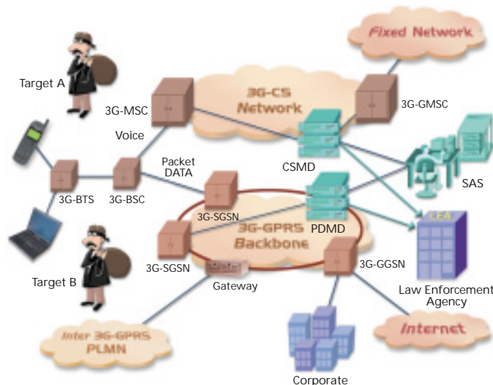
STAR-GATE Solution for Packet Data Networks
